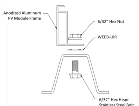
FIGURE 6: GROUNDING USING WEEB-UIR
